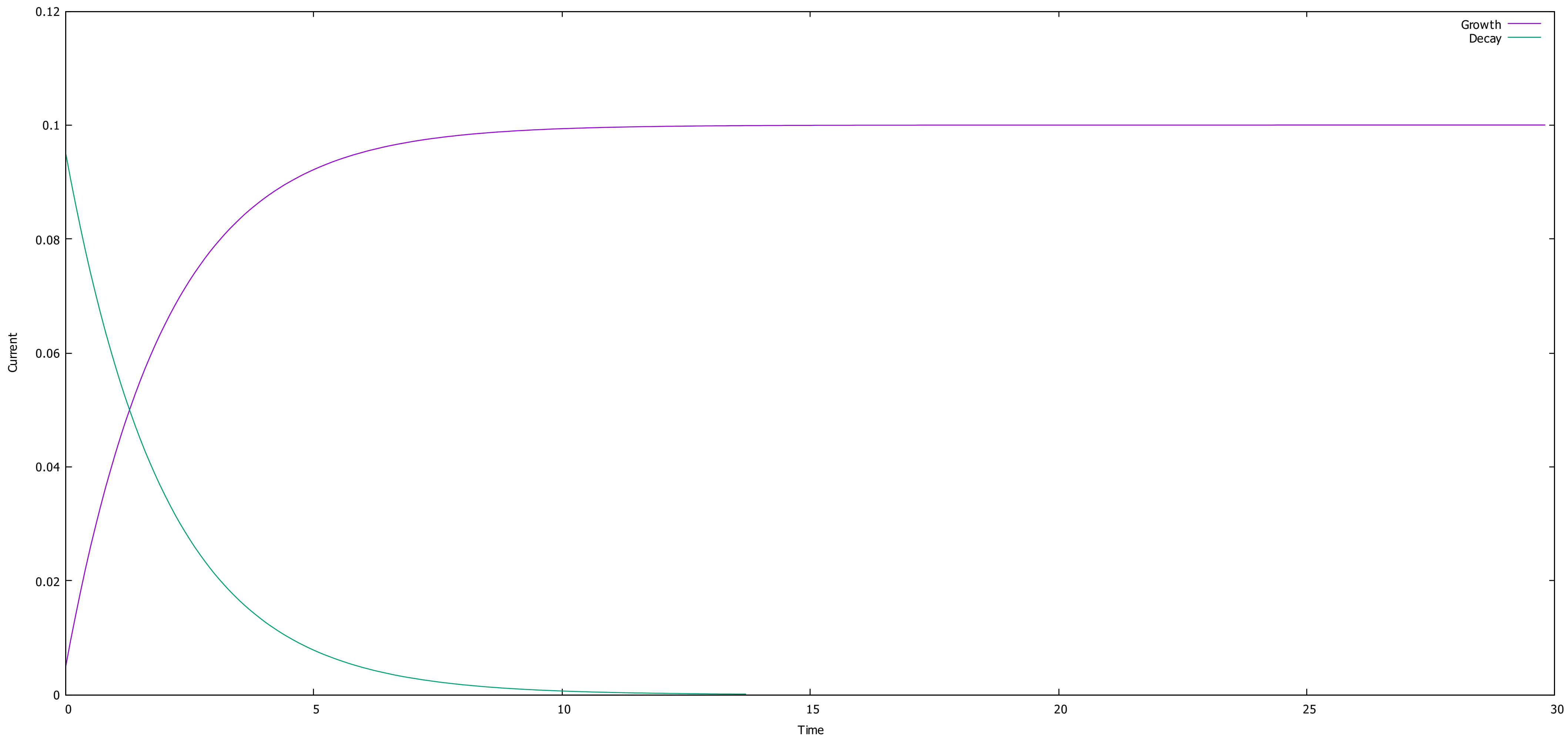
Growth and Decay of Current in RL Circuit using DC Source
